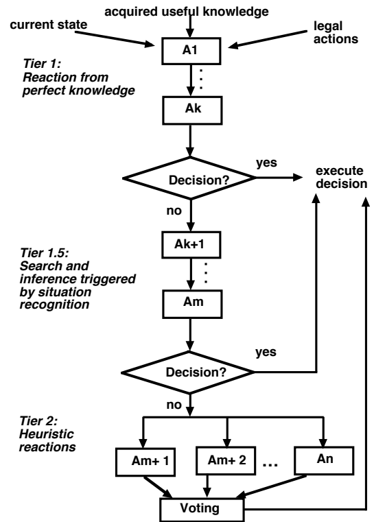
Figure 1: How FORR makes decisions.
