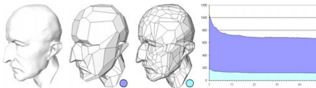
Figure 10: Max Planck : For the two optimized approximations (130 and 300 proxies resp.), we show the associated curves of the \mathcal{L}^{2,1} -distortion error as a function of Lloyd’s iterations; as expected, a few iterations suffice to reach a much reduced distortion error.
