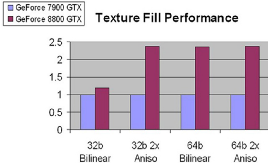
Figure 27. Texture fill performance of GeForce 8800 GTX
