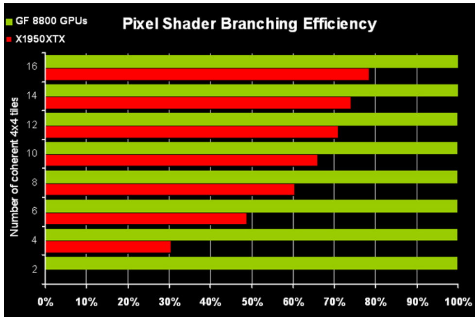
Figure 23. GeForce 8800 GPU pixel shader branching efficiency
