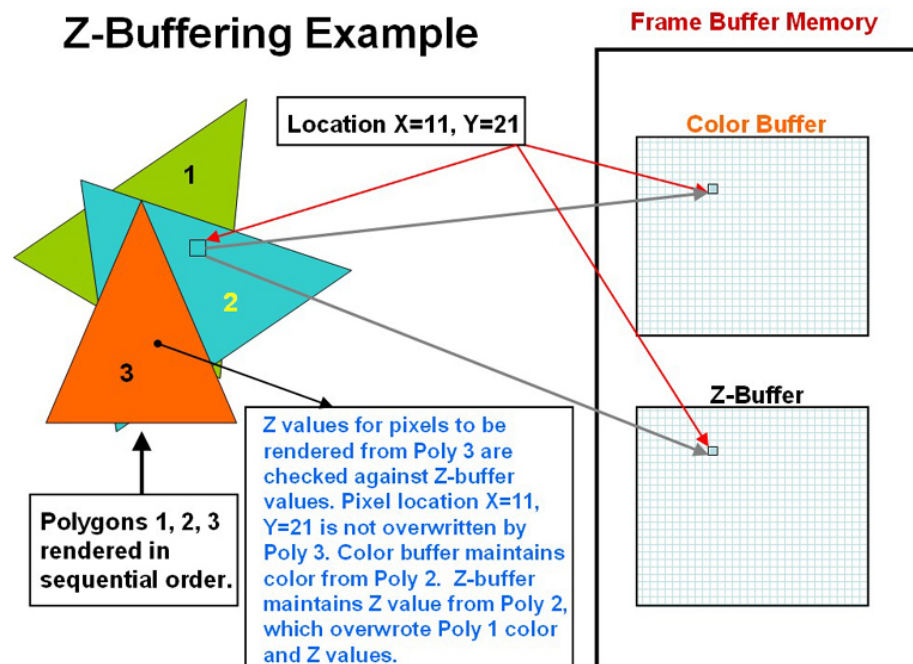
Figure 24. Example of Z-buffering
