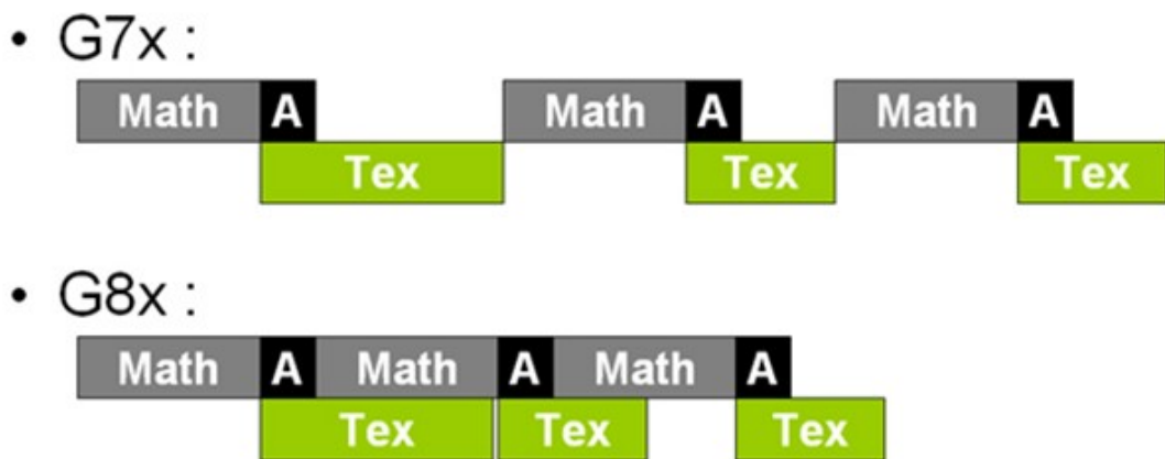
Figure 22. Decoupling texture and math operations
