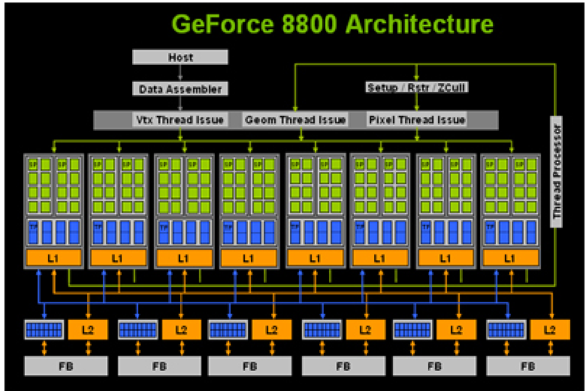
Figure 1. GeForce 8800 GTX Block Diagram
