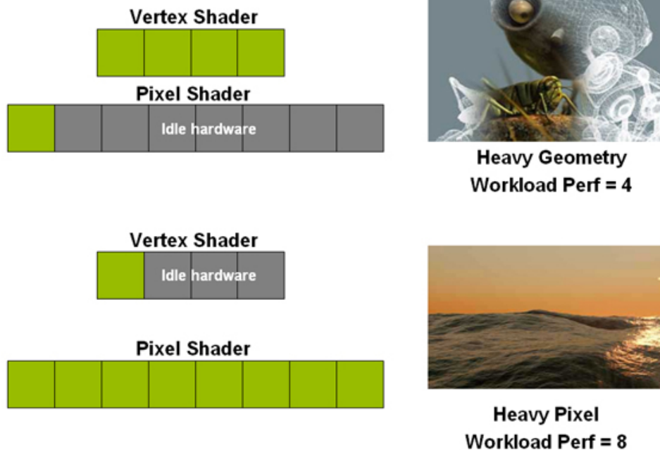
Figure 15. Fixed shader performance characteristics
