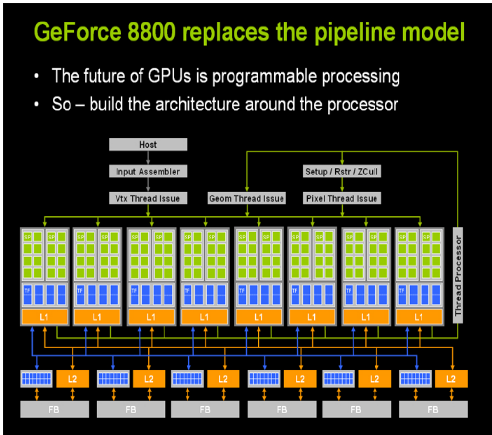
Figure 12. GeForce 8800 GTX block diagram
