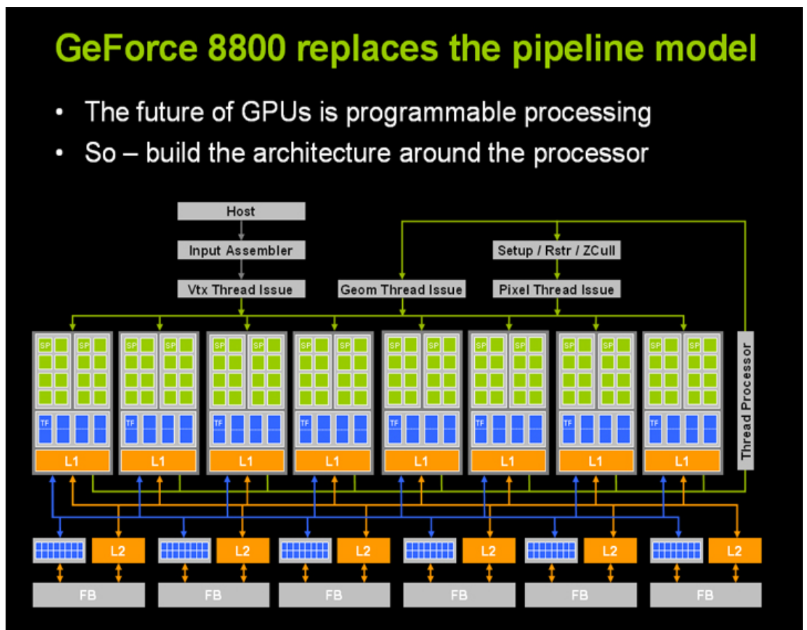
Figure 26. GeForce 8800 GTX block diagram
