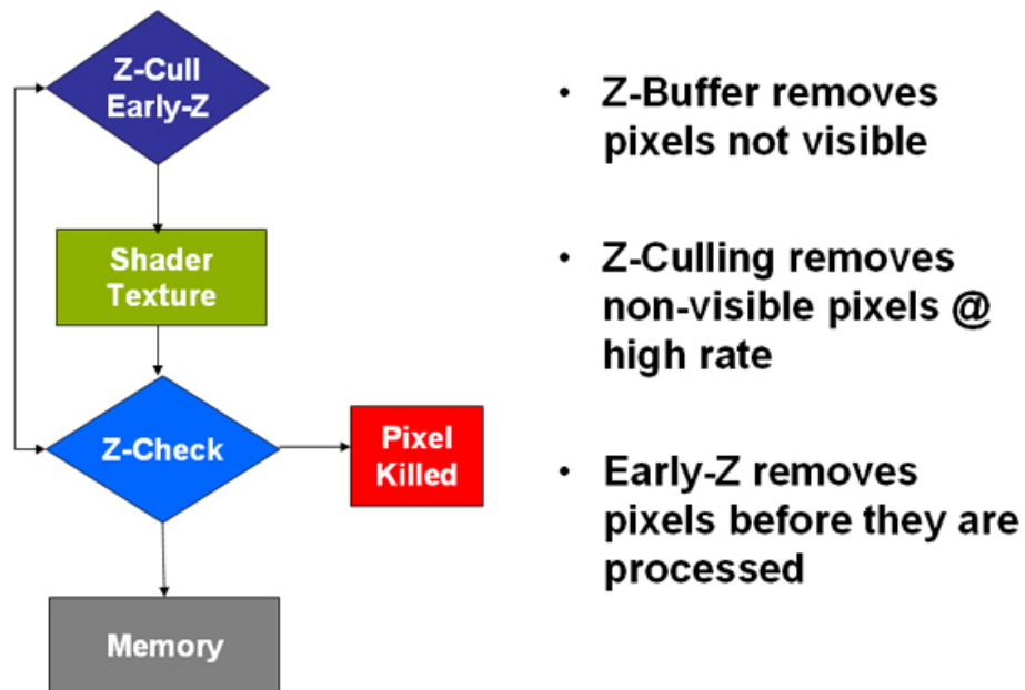
Figure 25. Example of early-Z technology
