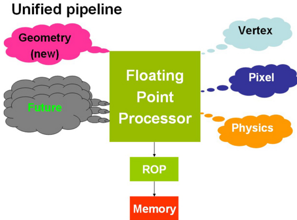
Figure 17. Conceptual unified shader execution framework
