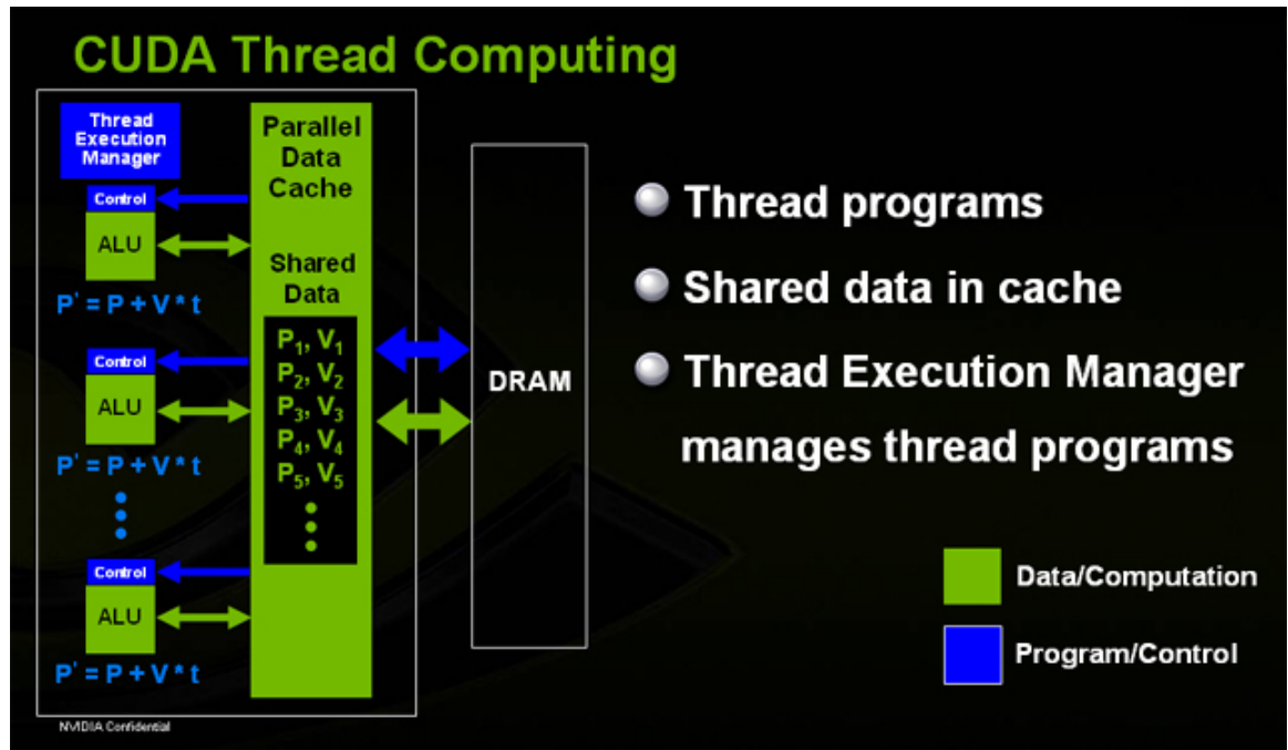
Figure 10. CUDA thread computing parallel data cache
