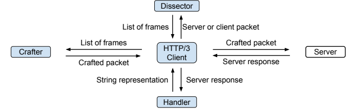
Fig. 7: Overview of Q3Fuzz fuzzing client
