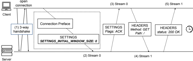
Fig. 6: CVE-2023-43622 vulnerability exploitation [4]
