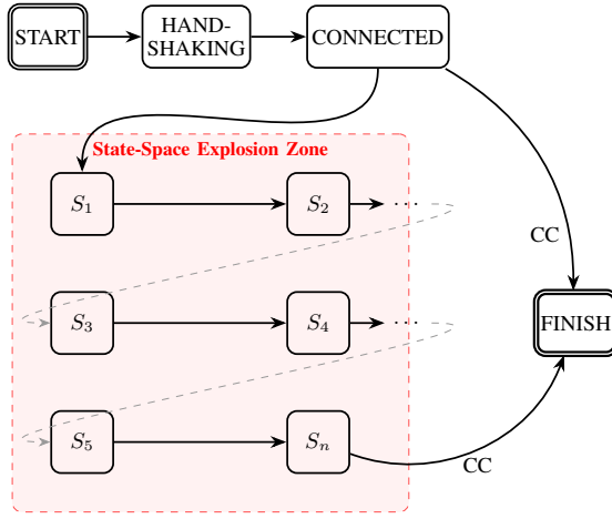
Fig. 9: Abstracted FSM depicting an example State Space Explosion due to nondeterministic server behavior. ( S_1 \rightarrow \dots \rightarrow S_n ).
