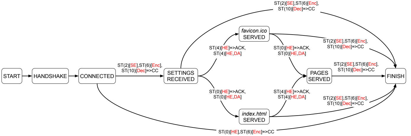
(b) Mvfst+Proxygen State Machine (simplified)
