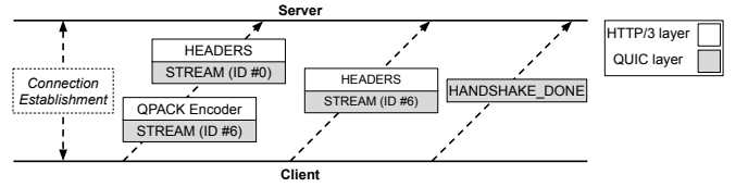
Fig. 2: Attack vector discovered by Q3Fuzz to crash a remote Proxygen server
