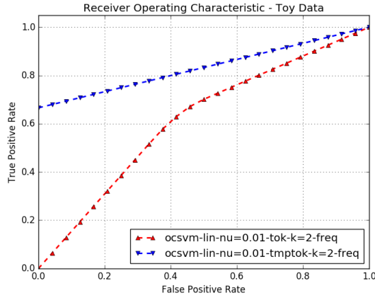
Fig. 3. Detection accuracy - temporal token features
