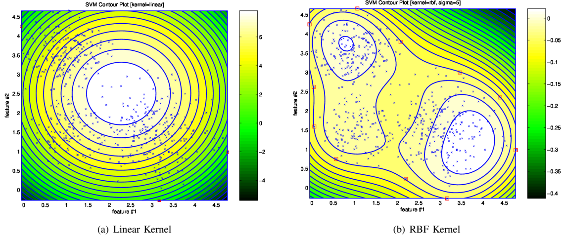
Fig. 2. Learning and anomaly detection using OC-SVM - Example data models obtained over synthetic data (red squares represent support vectors constituting the data model by defining the decision surface for separation between normal data and outliers.))
