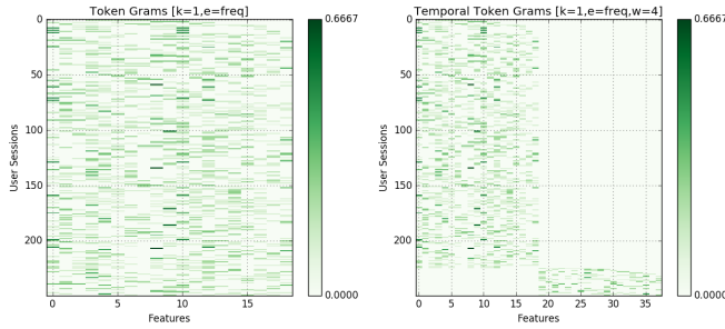
Fig. 4. 1-gram feature map - token grams (left) vs. temporal token grams (right)
