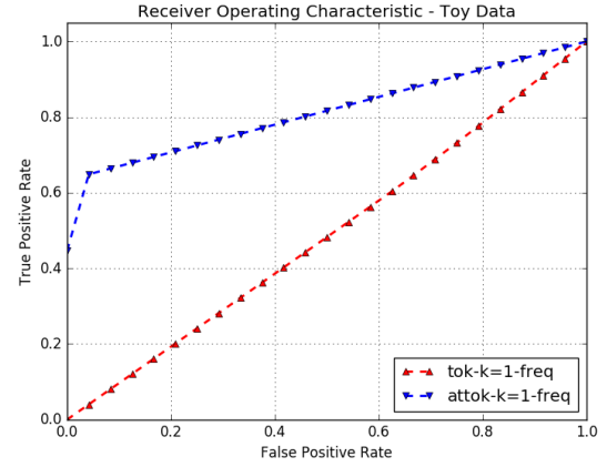
Fig. 5. Detection accuracy - attributed token features
