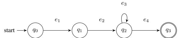
Fig. 1. Example of a user session graph with activity loop
