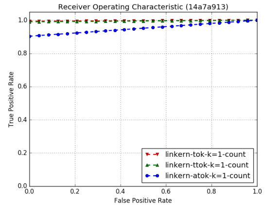
Fig. 6. Detection accuracy - User “14a7a913” (non-technical user)
